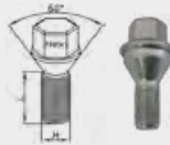
BOLT 60° BULLONE 60° (stainless steel cap)
