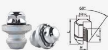
NUT 60° CLOSED DADO 60° CHIUSO
